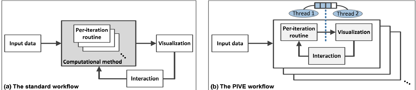
Figure 1: PIVE workflow (in comparison to a standard one). In the standard approach (a), the interactive visualization with a computational method is performed only after algorithm iterations finish. In contrast, PIVE (b) breaks up the computational method into per-iteration routines, allowing real-time interactive visualization with the intermediate output from algorithm iterations. To avoid overhead computations, PIVE divides the entire process into two concurrent threads (blue ellipses) linked with a message queue (blue rectangles).
